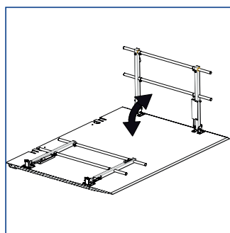
Guard hinged and folding on platform.
