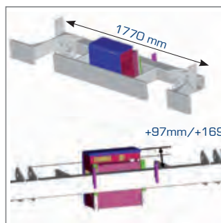
19 F3CL080 - Power pack inside rear bumper for narrow bodies.
