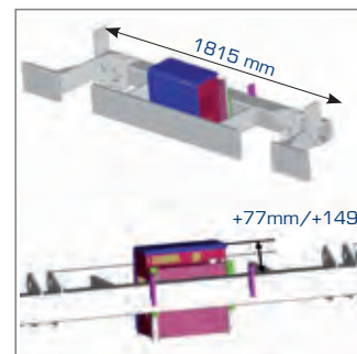
20 F3CL10 - Power pack inside rear bumper for narrow bodies.
