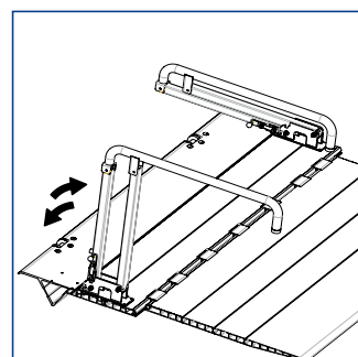
Pantograph safety gate
